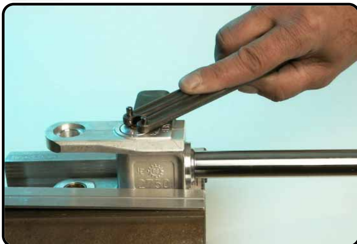
Disassemble the screw-cap rebound adjustment holder with T1218.
