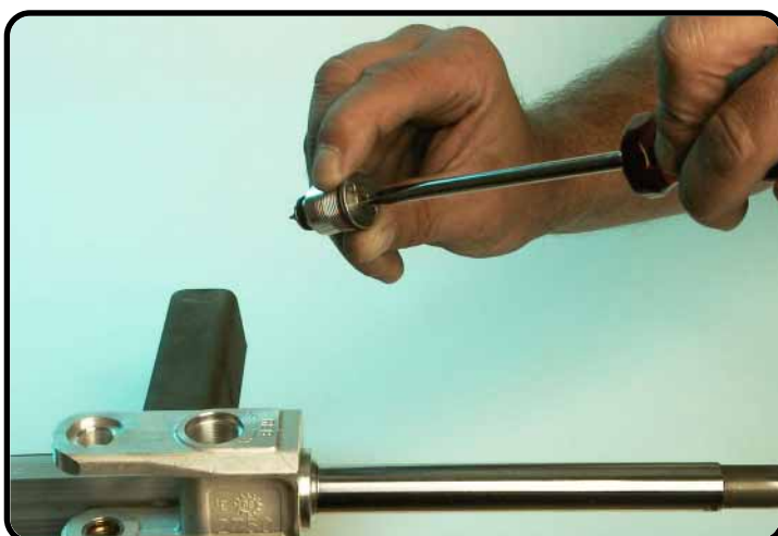
Unscrew the adjustment needle out of the adaptor.
